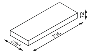
CRM28 post cap / wall cap
