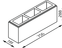
RM19 post block / wall block
