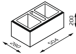
BH28 post block / wall block
