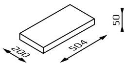
CH20, CRP20, CRD20 post cap / wall cap
