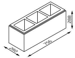
RM28 post block / wall block
