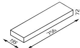
CRM19 post cap / wall cap
